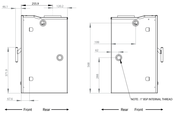
Boiler connections - Side view
