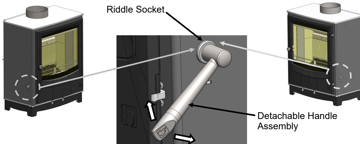
Fig. 6. Riddle Lever
