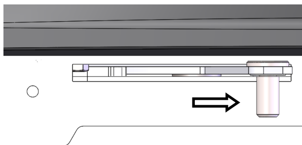
Fig. 3. Fully Open Position
