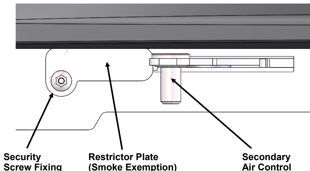
Fig. 6. Fitted Smoke Exemption Restrictor Plate
