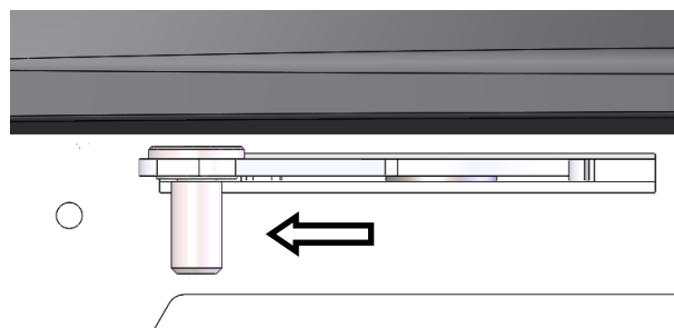
Fig. 4. Closed / Reduced Position
