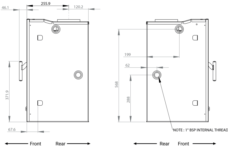
Boiler connections - Side view
