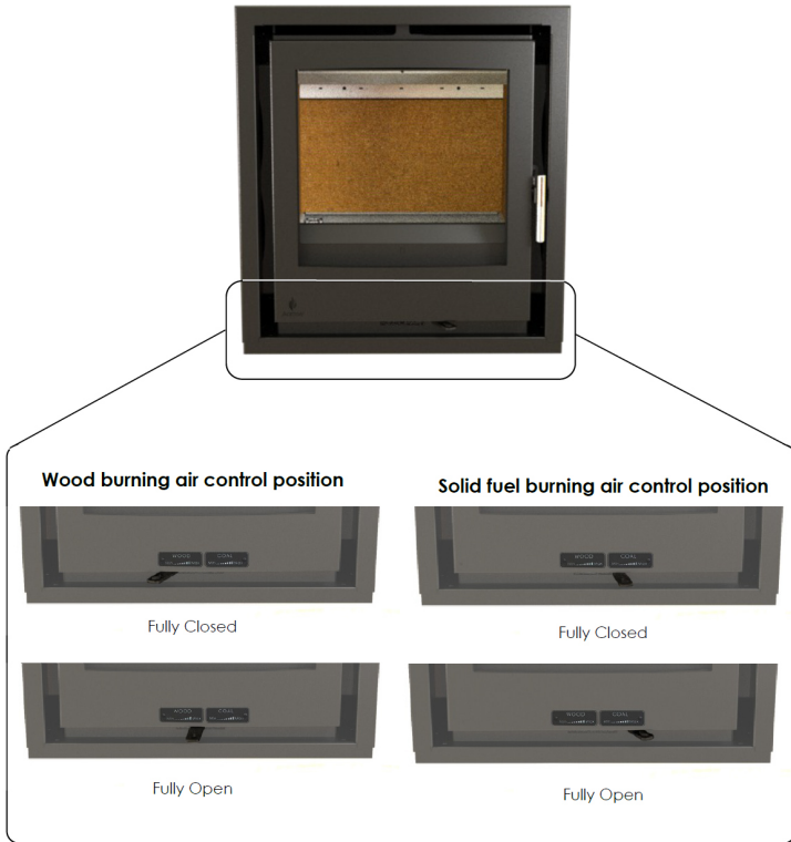
Figure2: i Series air inlet controls.
