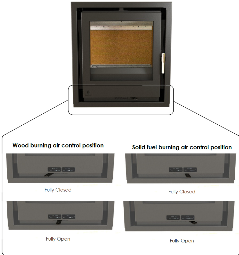
Figure 2: i Series air inlet controls.
