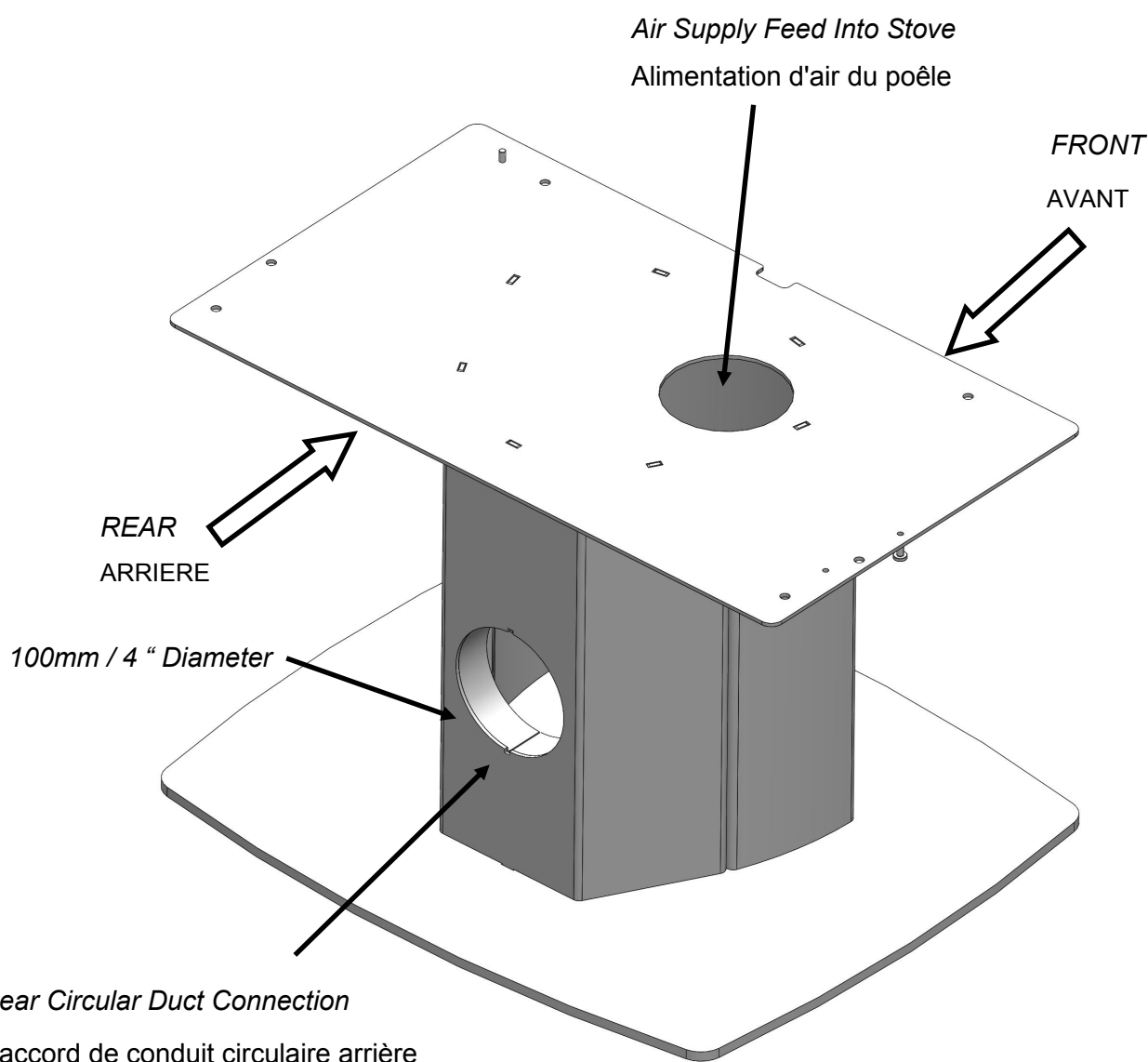
Farrington Pedestal Assembly (Looking At Rear of Unit) Piédestal de Farrington (Vue arrière)
